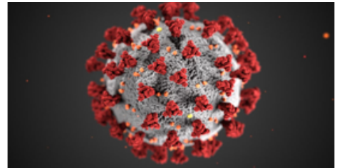
Coronavirus covid-19
